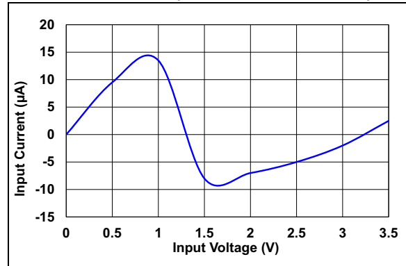
FIGURE 3-11: INPUT CURRENT VS. INPUT VOLTAGE ( V_{CC} = 3.3V , T_A = 25^\circ C )
