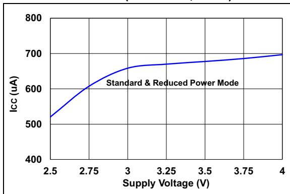
FIGURE 3-2: SUPPLY CURRENT VS. SUPPLY VOLTAGE – PIN-CONTROLLED POWER-DOWN MODE ( T_A = 25^\circ\text{C} , F = 0 )
