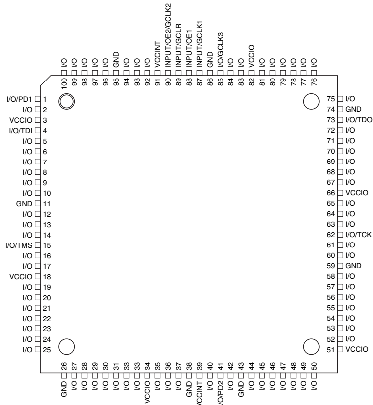
100-Lead TQFP (Top View)
