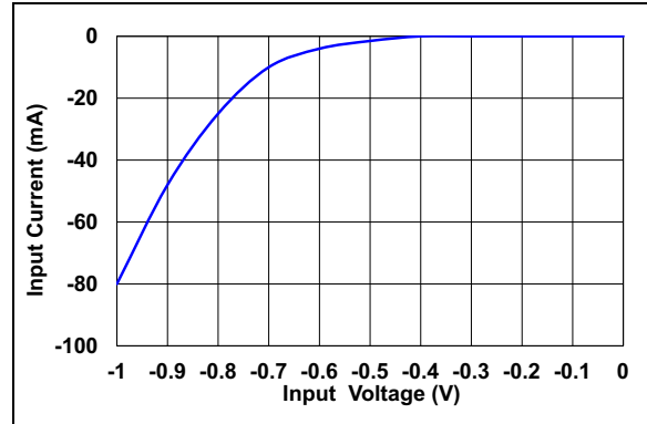
FIGURE 3-10: INPUT CLAMP CURRENT VS. INPUT VOLTAGE ( V_{CC} = 3.3V , T_A = 25^\circ C )
