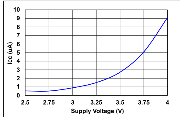
FIGURE 3-4: SUPPLY CURRENT VS. SUPPLY VOLTAGE – ATF1508ASVL ( T_A = 25^\circ\text{C} , F = 0 )
