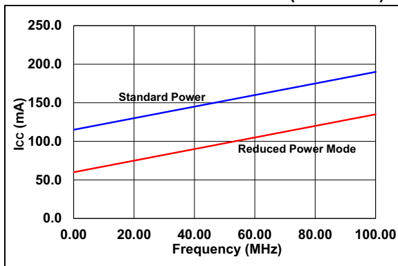
FIGURE 3-3: SUPPLY CURRENT VS. FREQUENCY – ATF1508ASV ( T_A = 25^\circ\text{C} )
