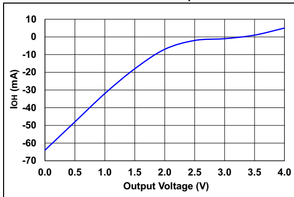
FIGURE 3-7: OUTPUT SOURCE CURRENT VS. OUTPUT VOLTAGE ( V_{CC} = 3.3V , T_A = 25^\circ C )
