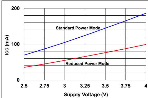
FIGURE 3-1: SUPPLY CURRENT VS. SUPPLY VOLTAGE – ATF1508ASV ( T_A = 25^\circ\text{C} , F = 0 )
