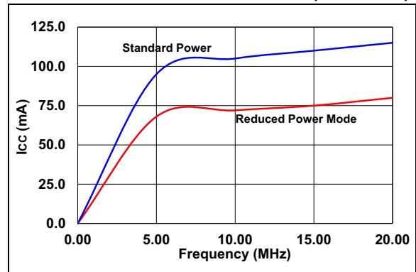
FIGURE 3-5: SUPPLY CURRENT VS. FREQUENCY – ATF1508ASVL ( T_A = 25^\circ\text{C} )
