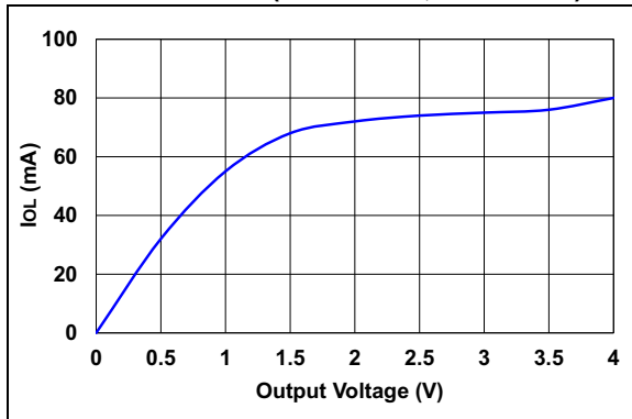
FIGURE 3-9: OUTPUT SINK CURRENT VS. OUTPUT VOLTAGE ( V_{CC} = 3.3V , T_A = 25^\circ C )
