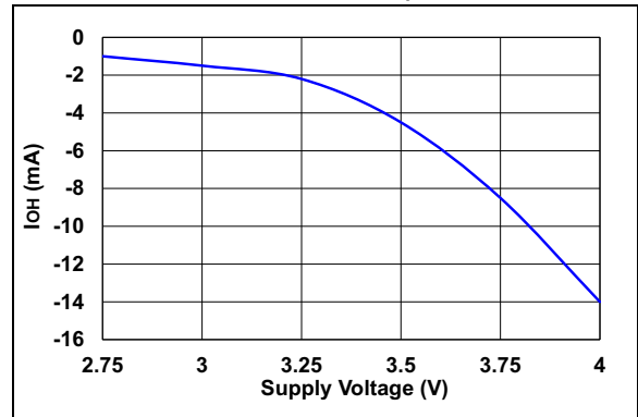
FIGURE 3-6: OUTPUT SOURCE CURRENT VS. SUPPLY VOLTAGE ( V_{OH} = 2.4\text{V} , T_A = 25^\circ\text{C} )
