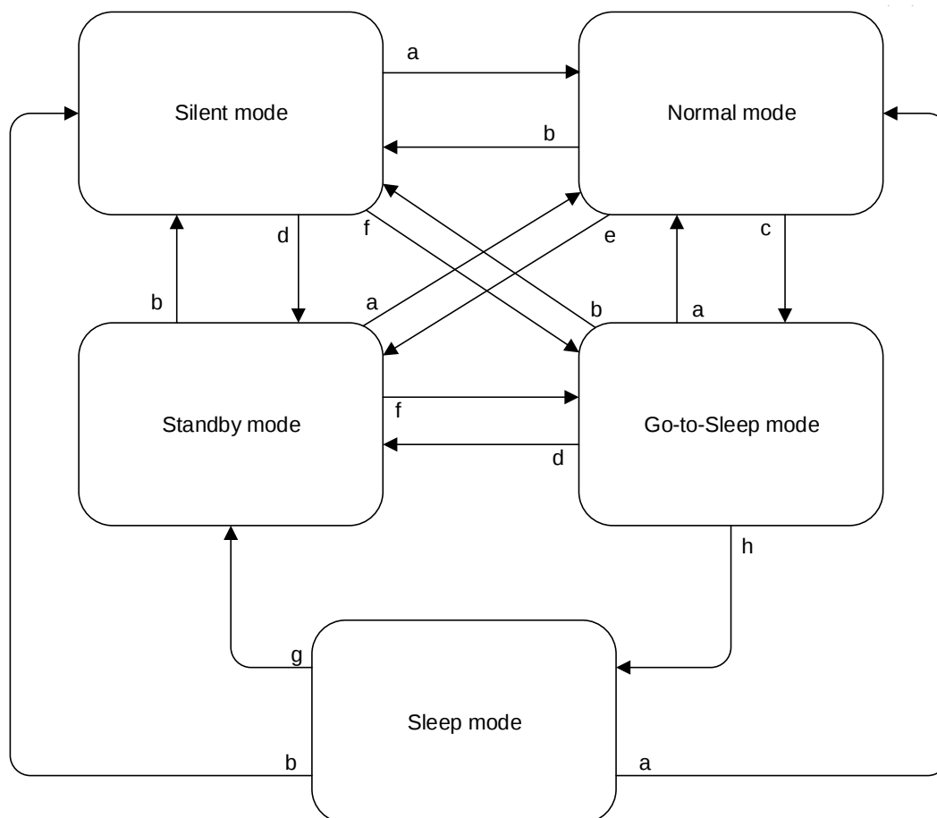
Figure 2-1. Operating Modes
