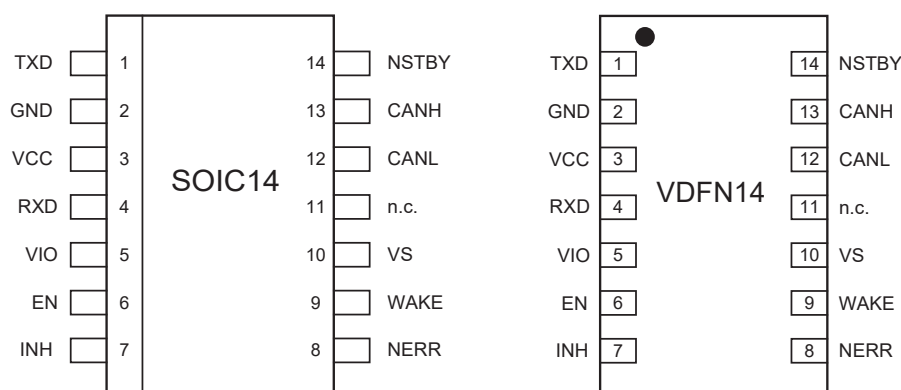
Figure 1-1. Pin Configuration
