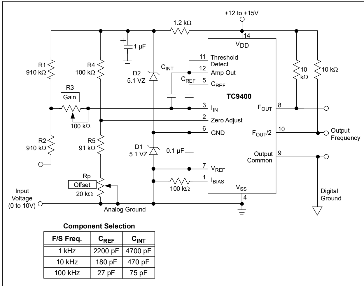
FIGURE 4-2: Voltage-to-Frequency.
