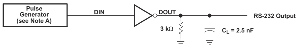
Figure 6-2. Driver Test Circuit and Waveforms for t_{PHL} and t_{PLH} Measurements (5- \mu s Input)
