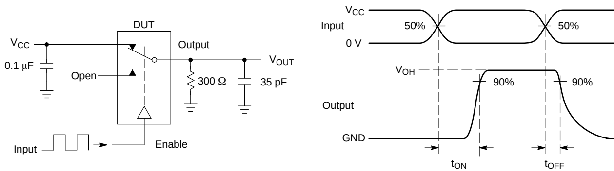
Figure 20. t_{ON}/t_{OFF}
